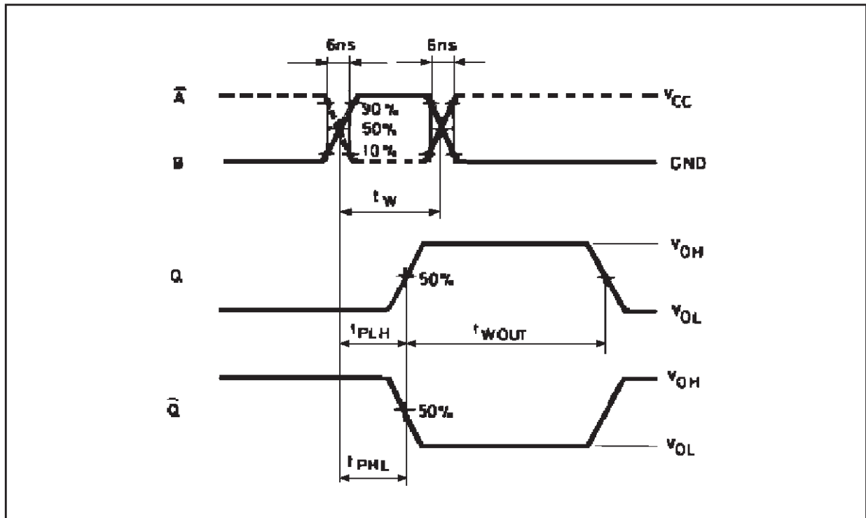
WAVEFORM 1: MINIMUM PULSE WIDTH ( \bar{A} , B), OUTPUT PULSE WIDTH, PROPAGATION DELAY TIME ( f=1\text{MHz} ; 50% duty cycle)
